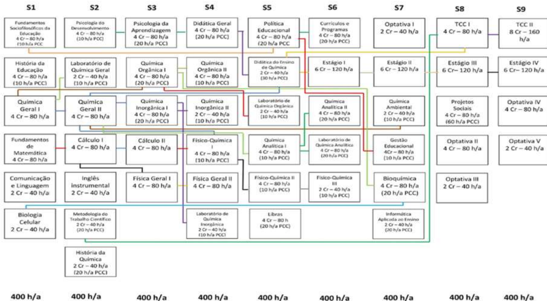
Figura 1. Fluxograma curricular.
